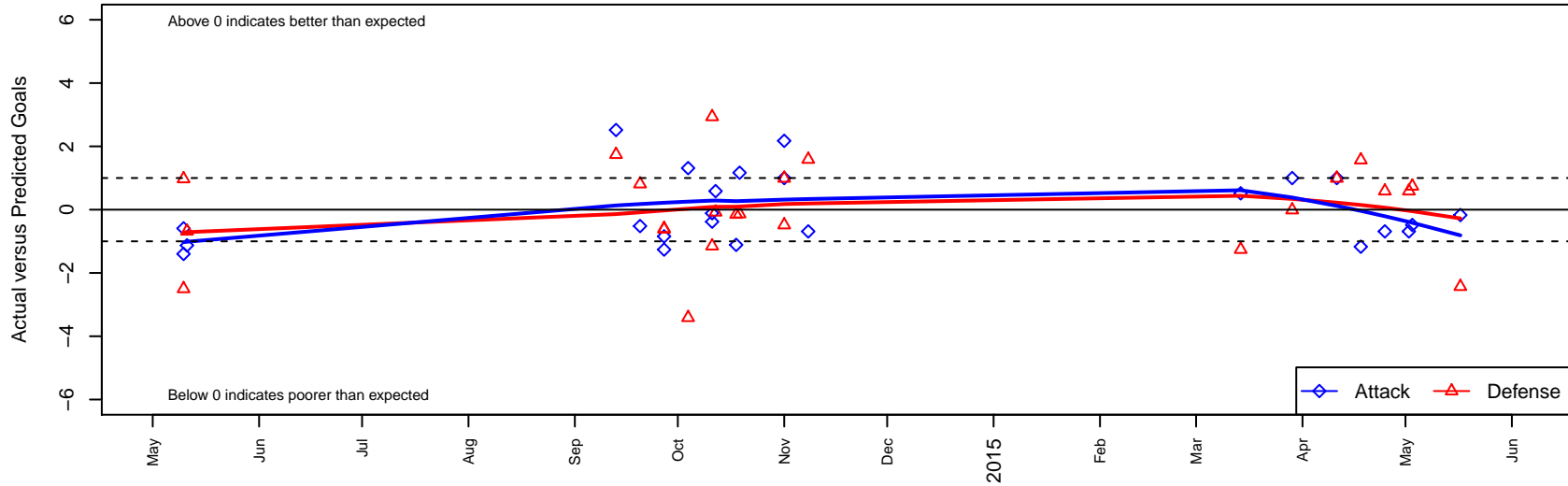
Valley Thunder SC G02 Dots are actual minus expected GF (blue circles) and GA (red triangles). Blue line is smoothed change in attack strength. Red is smoothed change in defense strength.
